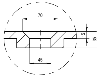
DETAIL D SCALE 1:3
